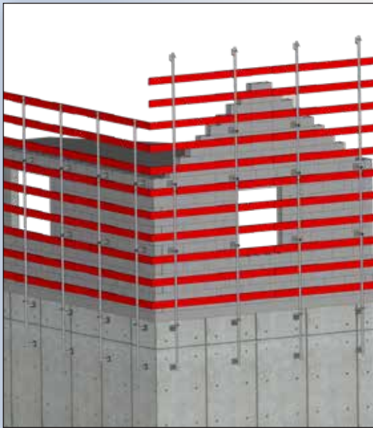
Montant 2,80 m Version planches
